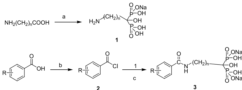
Scheme 1. Reagents: (a) H 3 PO 3 , PCl 3 ; (b) SOCl 2 ; (c) NaOH.
