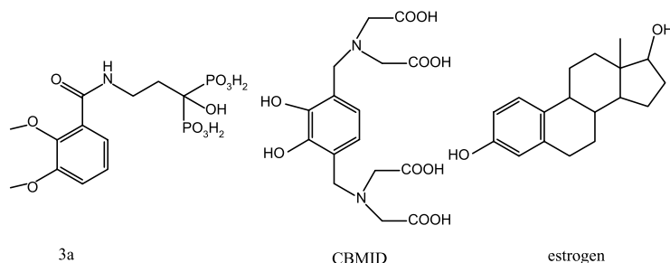
Figure 3. The structures of three anti-osteoporosis compounds.
